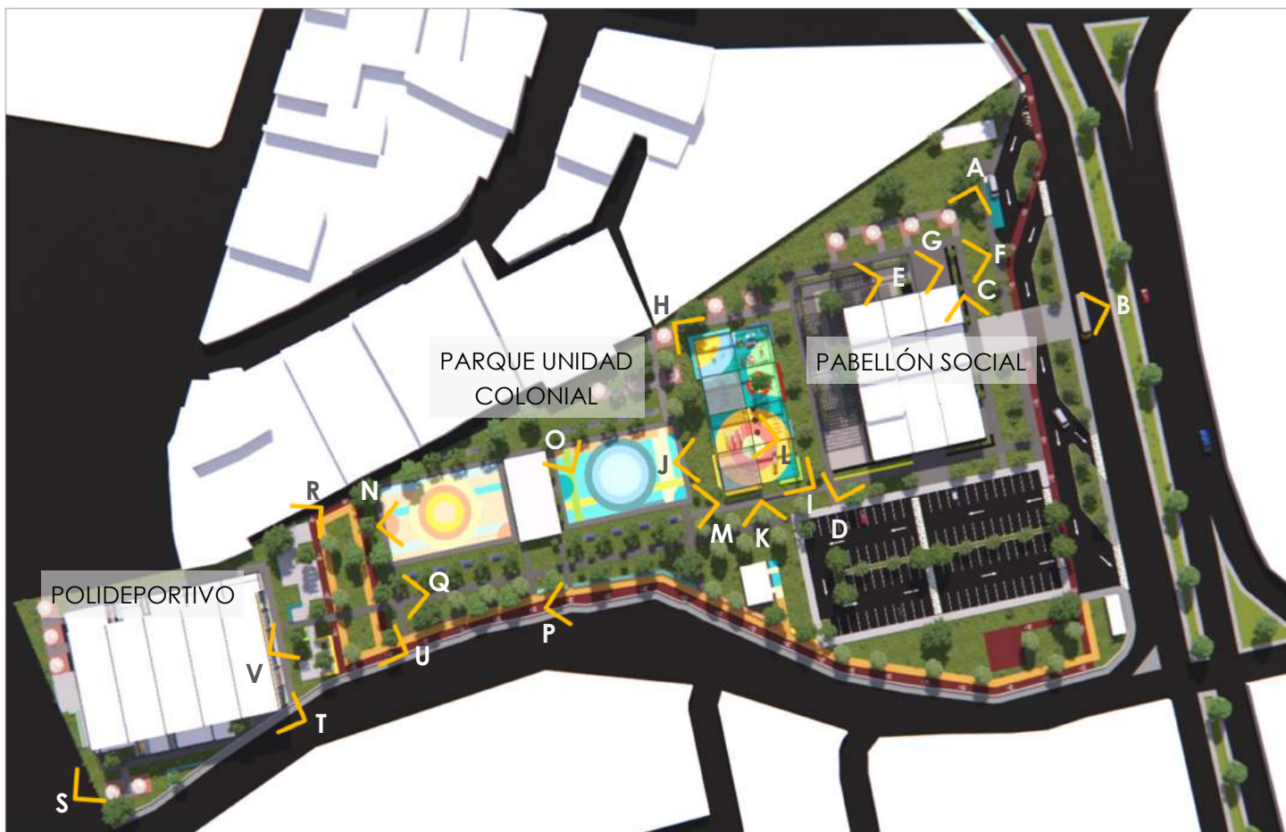
PLANTA, SOLAR 7
