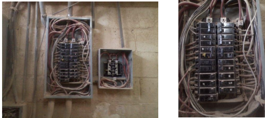
Figura 31. Acometida principal
