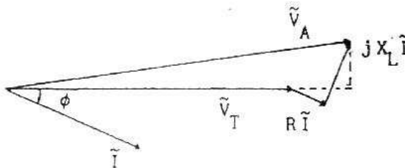
Figura 42. Diagrama Fasorial
