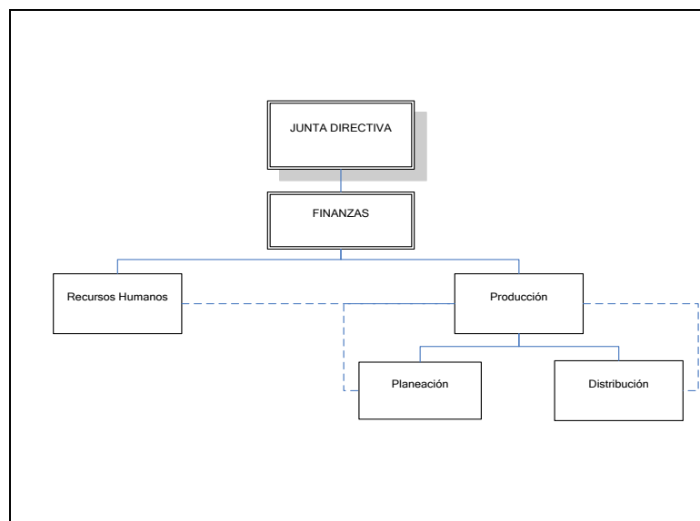
Figura 1. Organigrama
