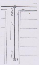
PLANTA PV-DP-7 A PV-DP-8 TRAMO 3 E.C. 1: 500
